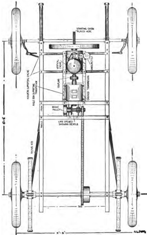
FIG. 415.—Plan diagram of the "Dyke" 6 H. P. Tonneau Carriage, showing position of the working parts, as in Fig. 418.
